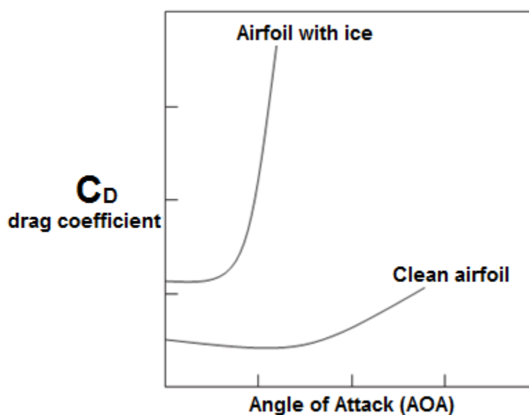
FIGURE 3-6. DRAG CURVE
