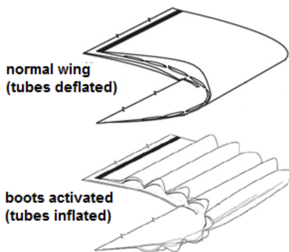
FIGURE 3-7. WING BOOT
