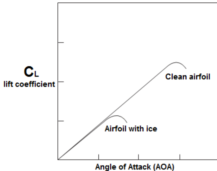
FIGURE 3-5. LIFT CURVE
