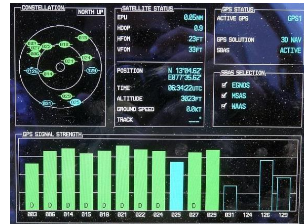
GPS status page showing PRN-identified satellites
